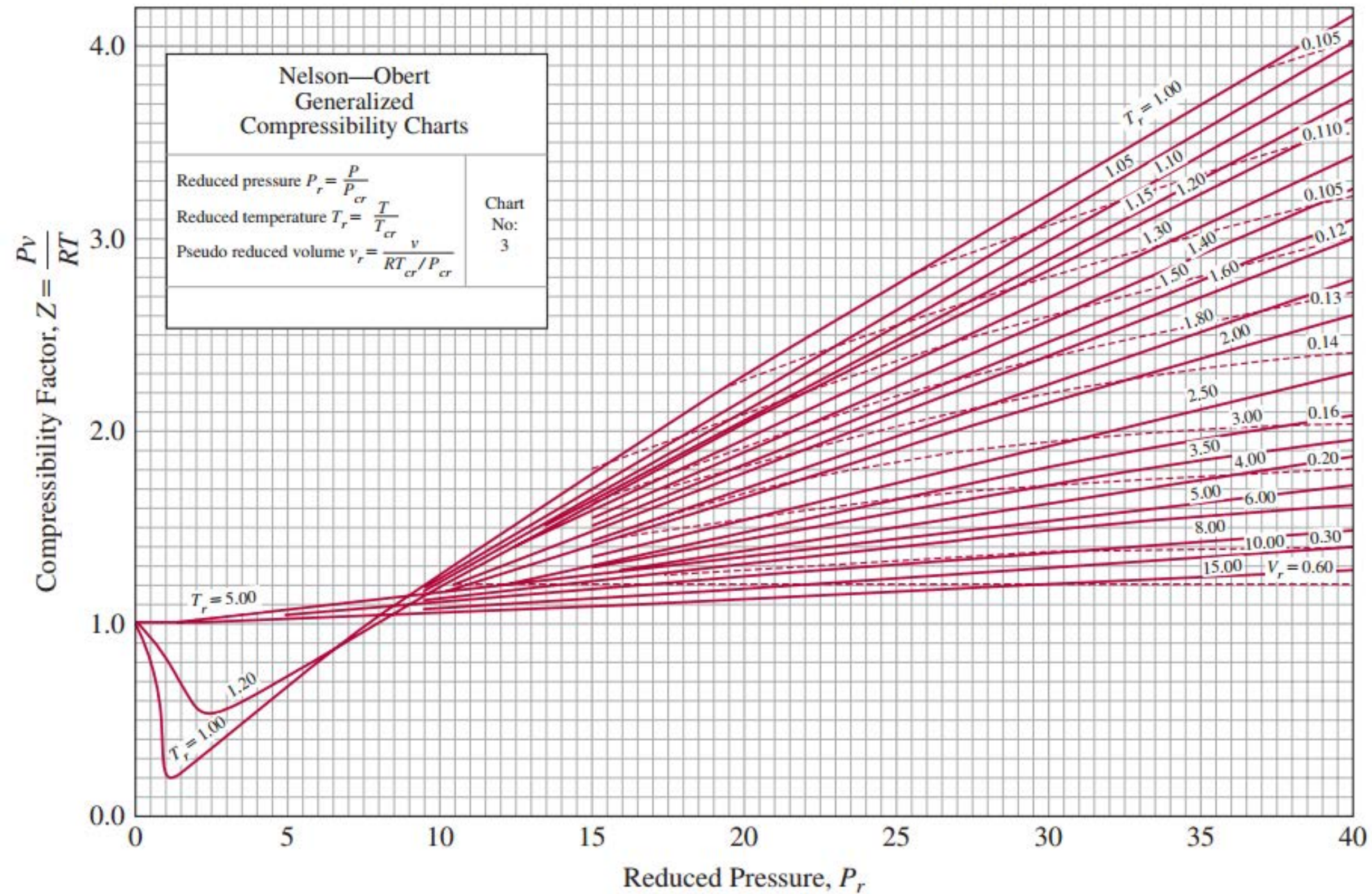
Nelson-Obert Generalized (Averaged) Compressibility Chart
